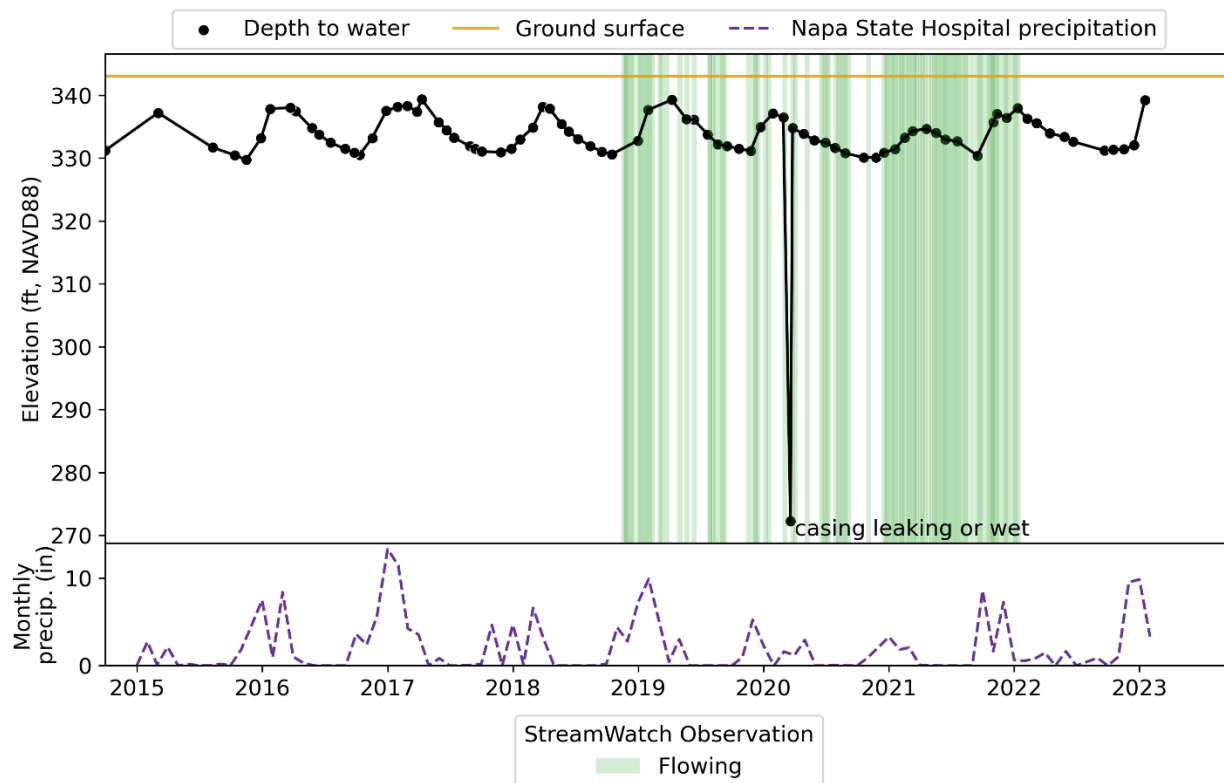
Figure 5-1. Groundwater levels in NapaCounty-128 monitoring well, observations at Stream Watch Site 11, and monthly precipitation at Napa State Hospital
