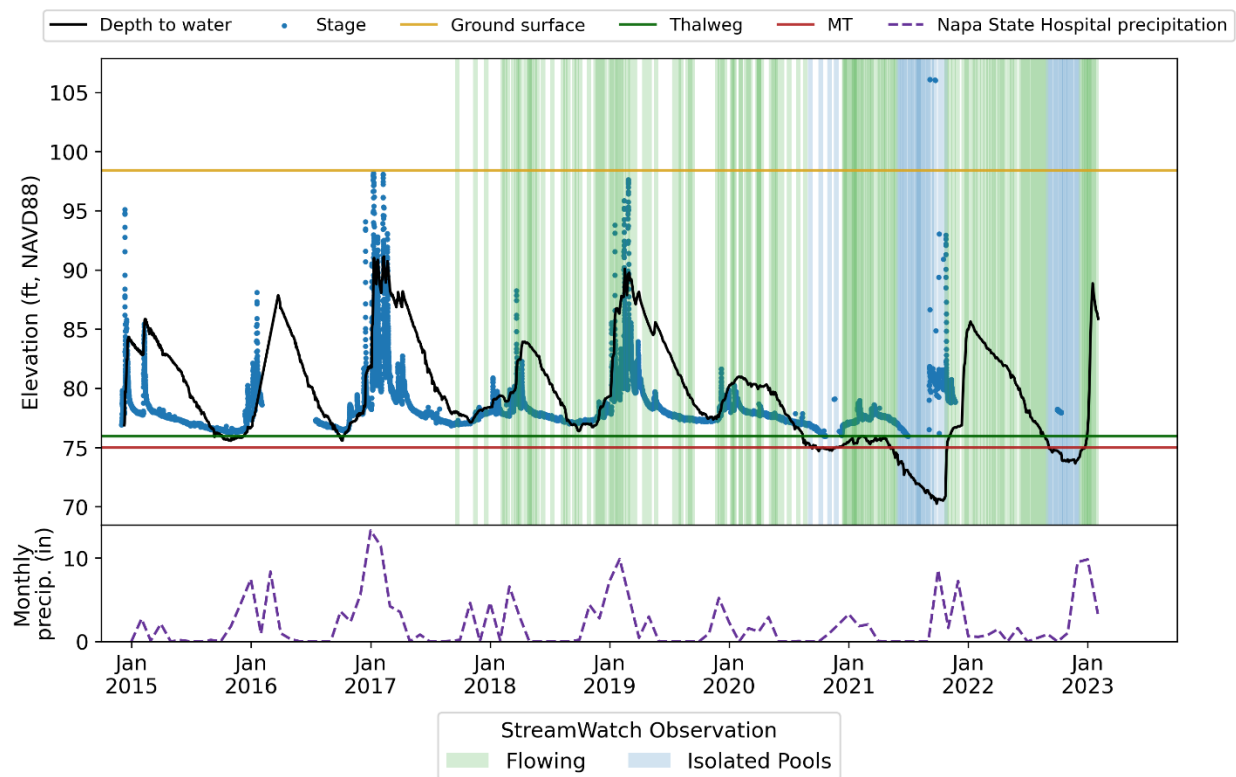
Figure 5-4. NapaCounty-220s-swgw4, groundwater levels and stage, observations from Stream Watch Site 1, monthly precipitation at Napa State Hospital, thalweg elevation near monitoring well, and the Minimum Threshold for monitoring well.
