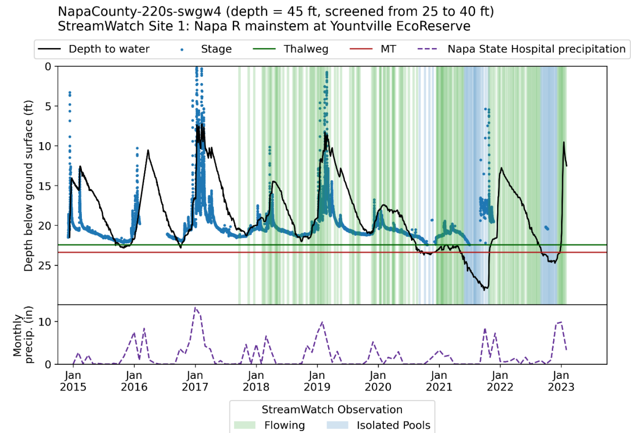
Figure 5-4. NapaCounty-220s-swgw4, groundwater levels and stage , observations from Stream Watch Site 1, monthly precipitation at Napa State Hospital, thalweg elevation near monitoring well, and the Minimum Threshold for monitoring well.
