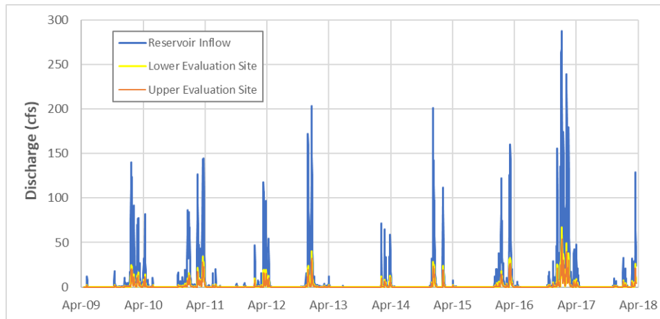
Figure 13: Total reservoir inflow and additional flow contributions to the Terroir (upper) and Vineyard (lower) evaluation sites as simulated with the hydrologic model.
