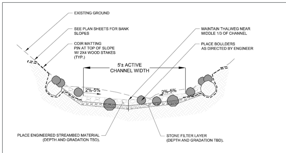
Figure 4. Typical Revegetation and Restoration of a Stream Section
